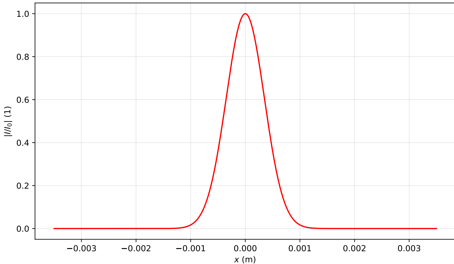
Intensity profile I(x, y = 0, z = 0.000)/I_0 , \text{Pin}=9.0\text{Pcr} , artificial time
